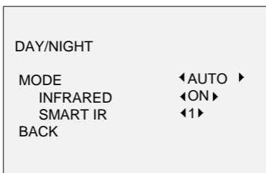
Figure 3-6 DAY NIGHT
