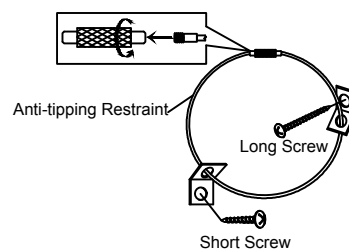
Anti-Tipping Device 1 set
