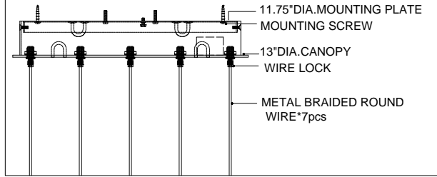
CANOPY DETAIL
