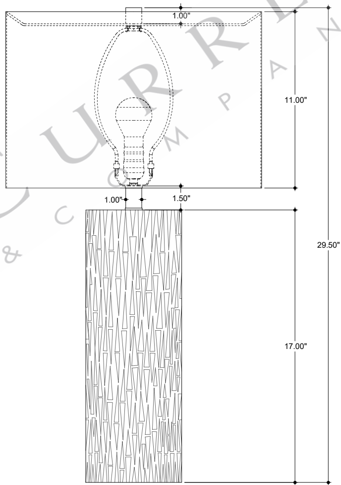
FRONT VIEW
