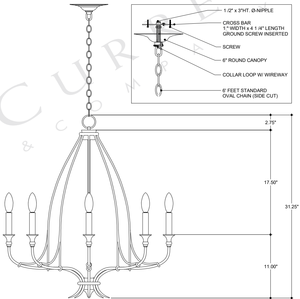
FRONT VIEW
