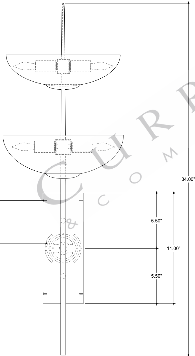
FRONT VIEW
