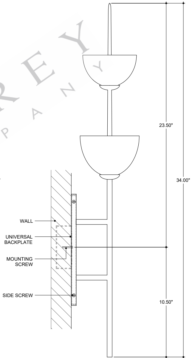
SIDE VIEW
