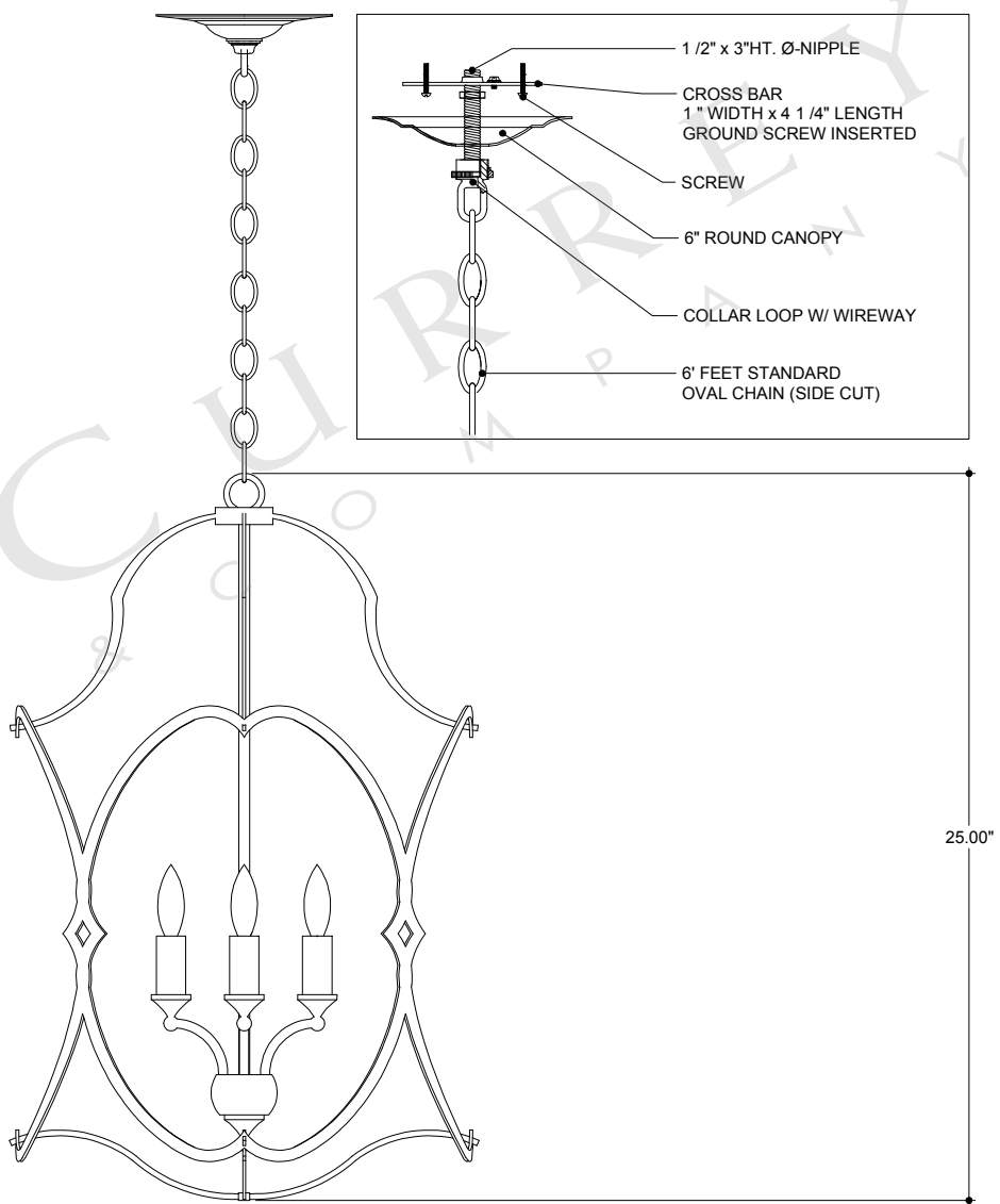
FRONT VIEW
