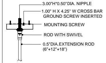
CANOPY DETAIL
