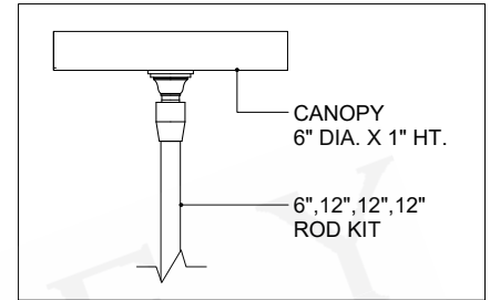
CANOPY DETAIL
