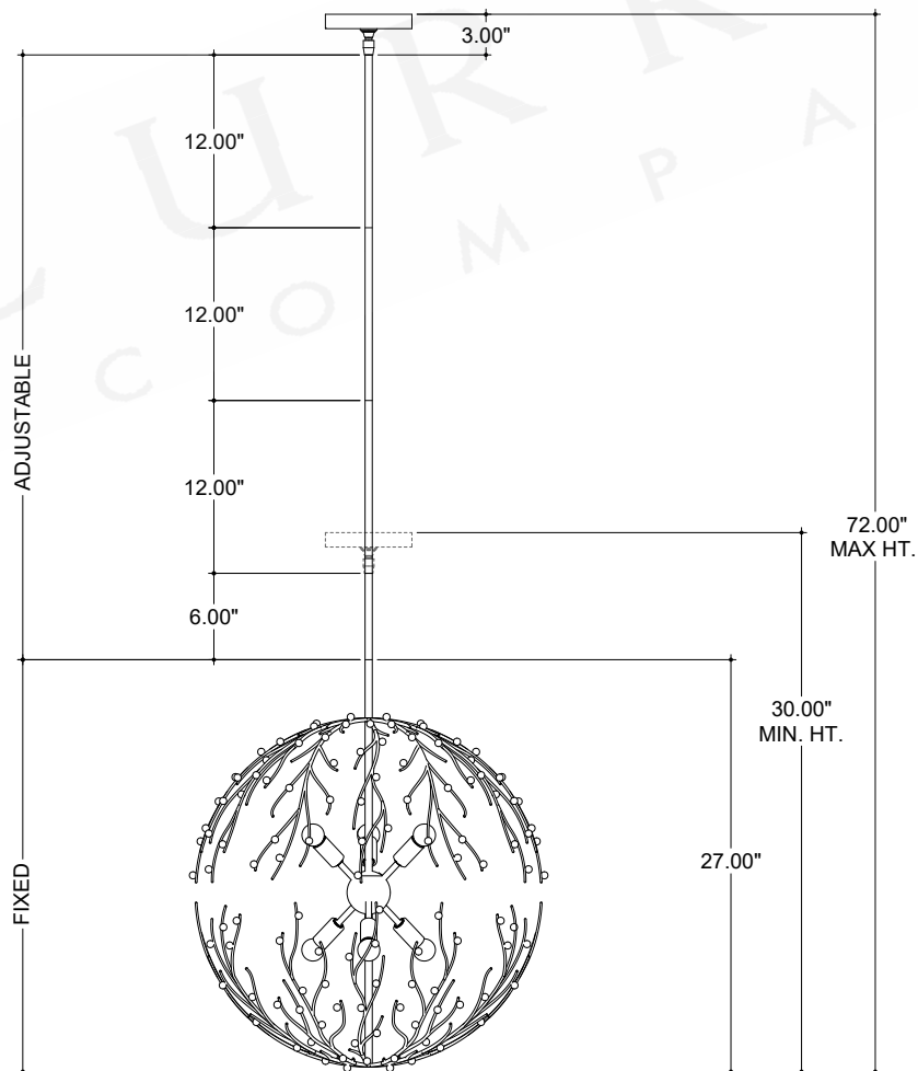
FRONT VIEW
