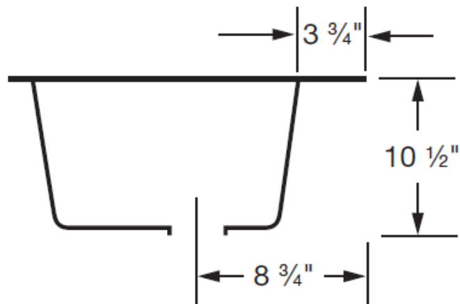
SSUS-S 17 \frac{1}{4}'' W x 20'' D (438 mm x 508 mm) A 14", B 14" Capacity: 7 gallons
