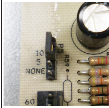
FIGURE 32 - JUMPER P5
