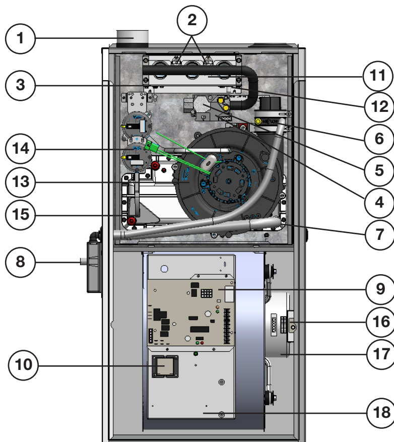
FIGURE 1 - FURNACE COMPONENTS
