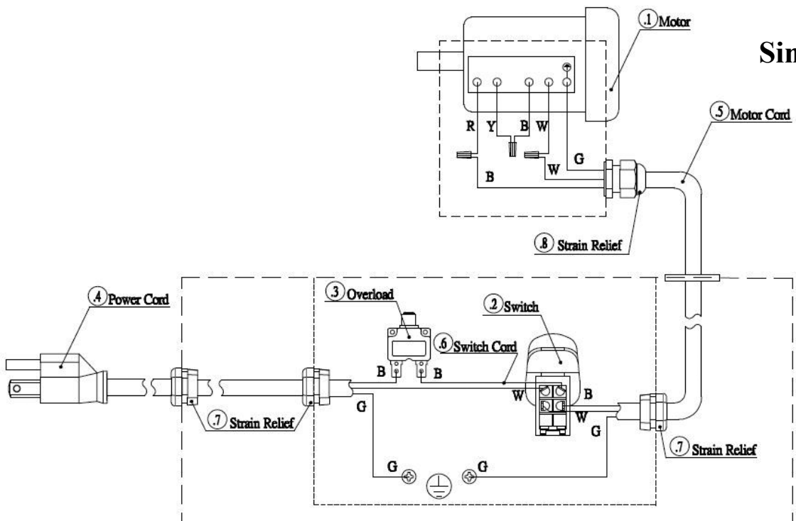
Figure 10 - 9681109 single phase 230 V electrical diagram.
