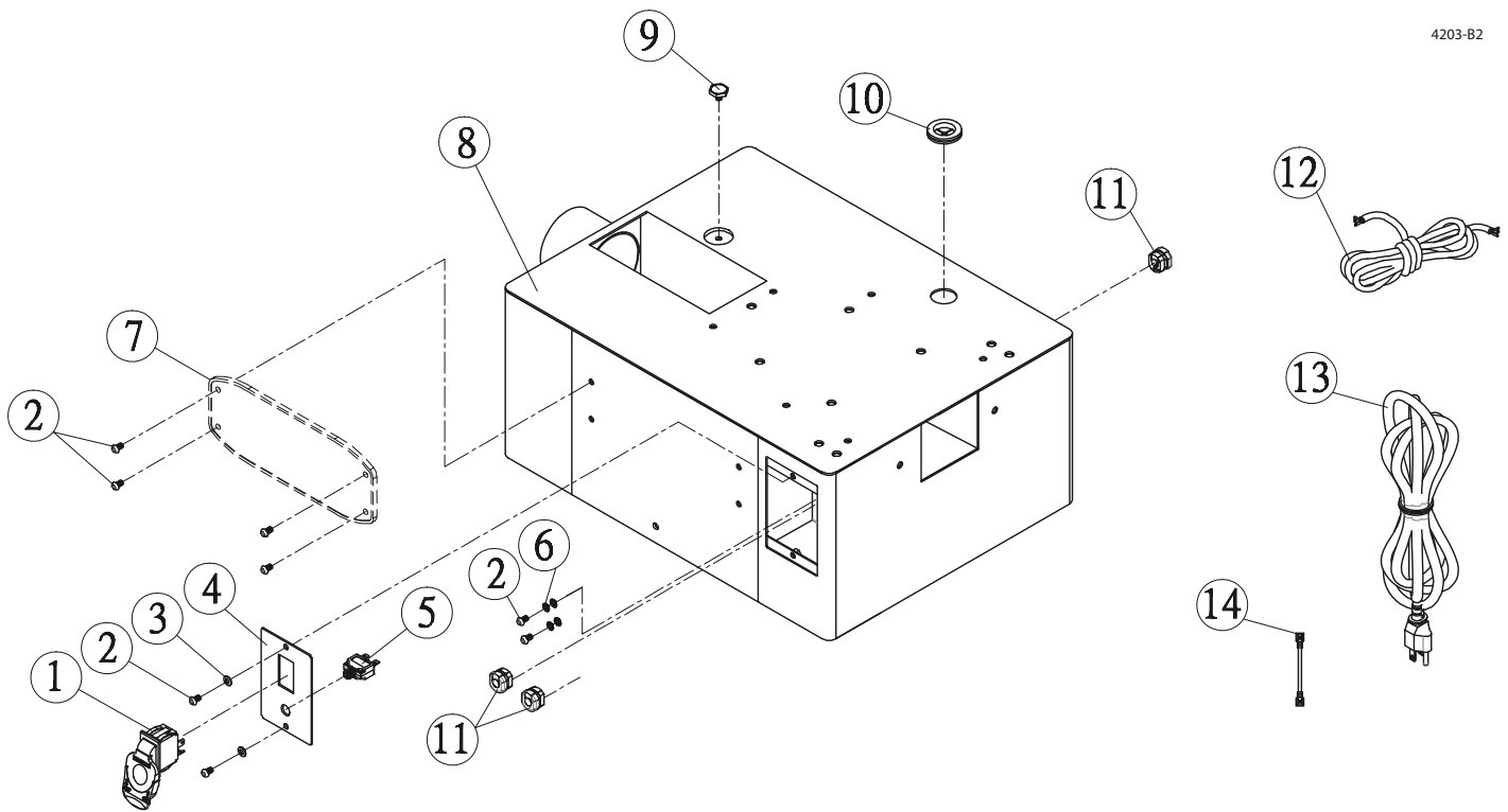
Figure 15 – Replacement Parts Illustration for 9681109 Base
