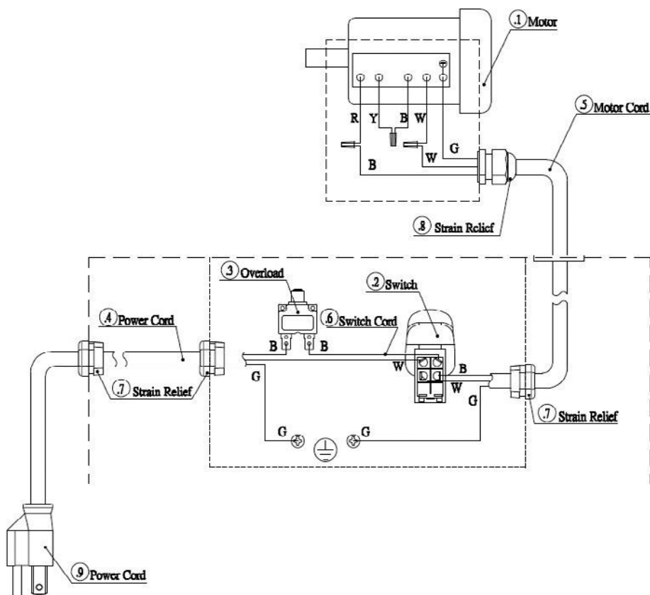
Figure 12 - 9681108 single phase 230V electrical diagram.
