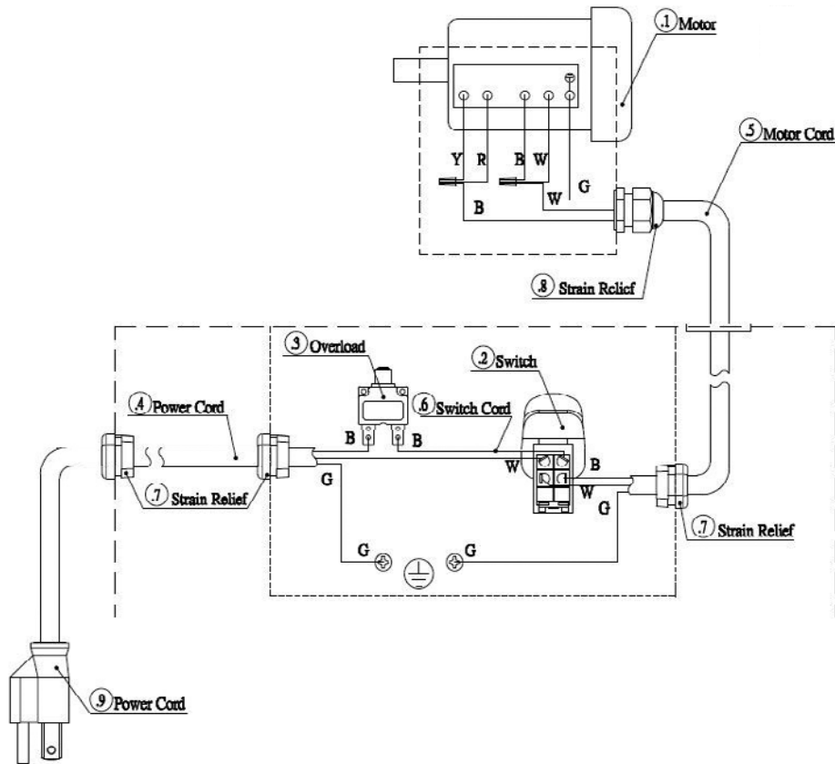
Figure 11 - 9681108 single phase 115V electrical diagram.
