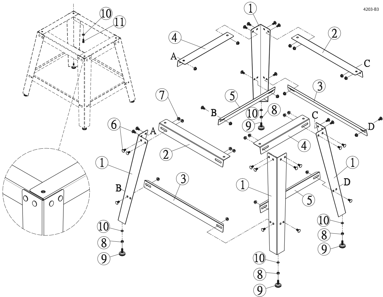
Figure 16 – Replacement Parts Illustration for 9681109 Stand
