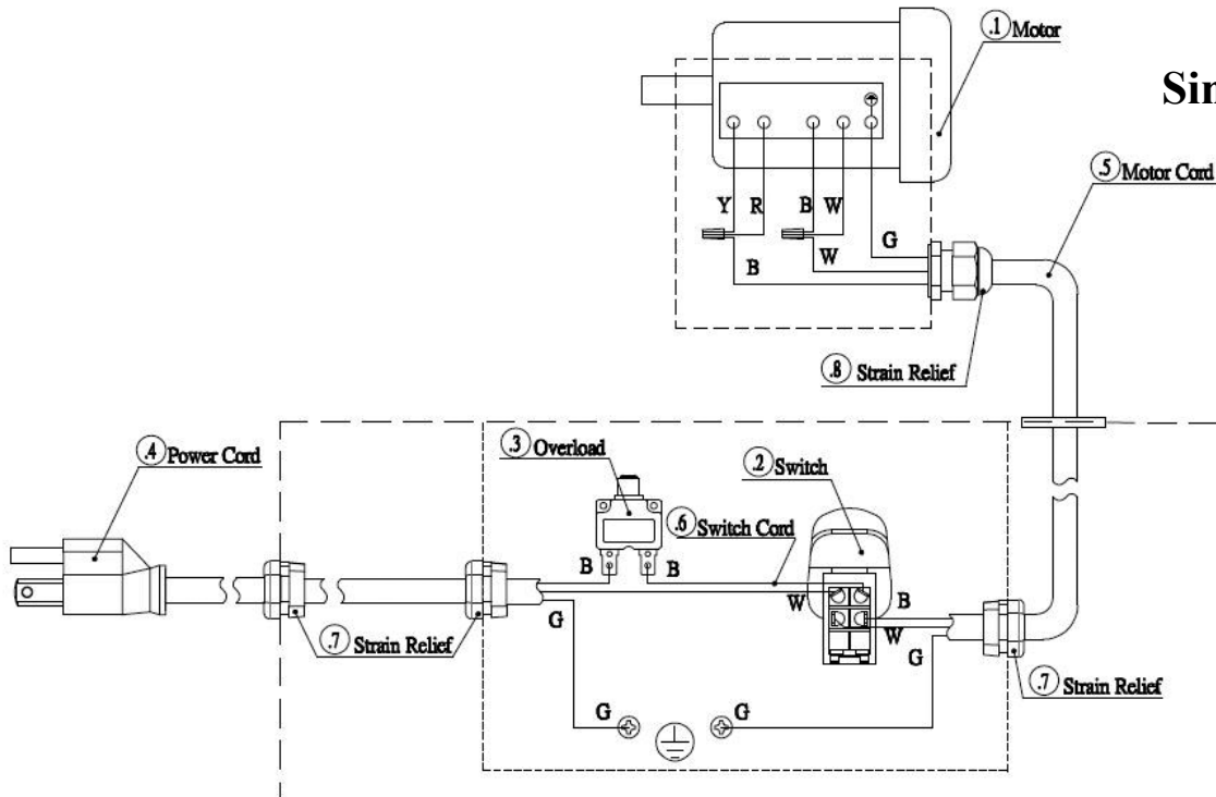
Figure 9 - 9681109 single phase 115 V electrical diagram.
