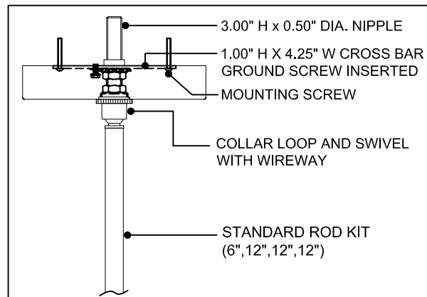
CANOPY DETAIL
