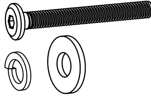
ALLEN KEY BOLT: M8 X 60mm - QTY 8 LOCK WASHER: \varnothing 12 / \varnothing 8 \times 1.5\text{mm} - QTY 8 WASHER: \varnothing 19 / \varnothing 8 \times 1\text{mm} - QTY 8
