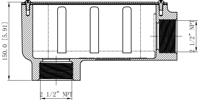
CUTAWAY VIEW A-A
