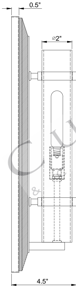
SIDE VIEW
