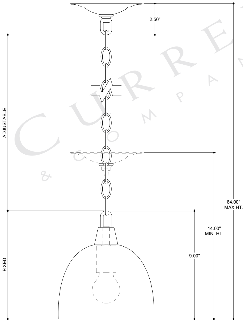
FRONT VIEW
