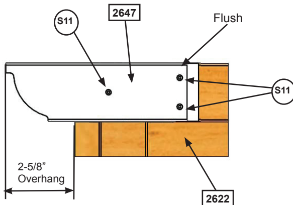
Fig. 41.5 Side View
