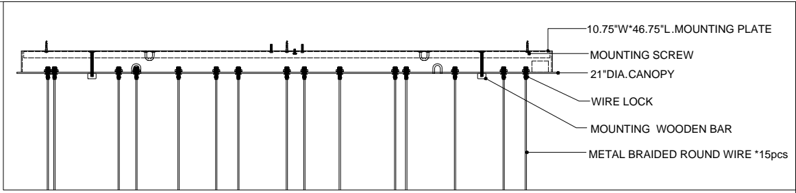
CANOPY DETAIL
