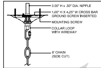
CANOPY DETAIL
