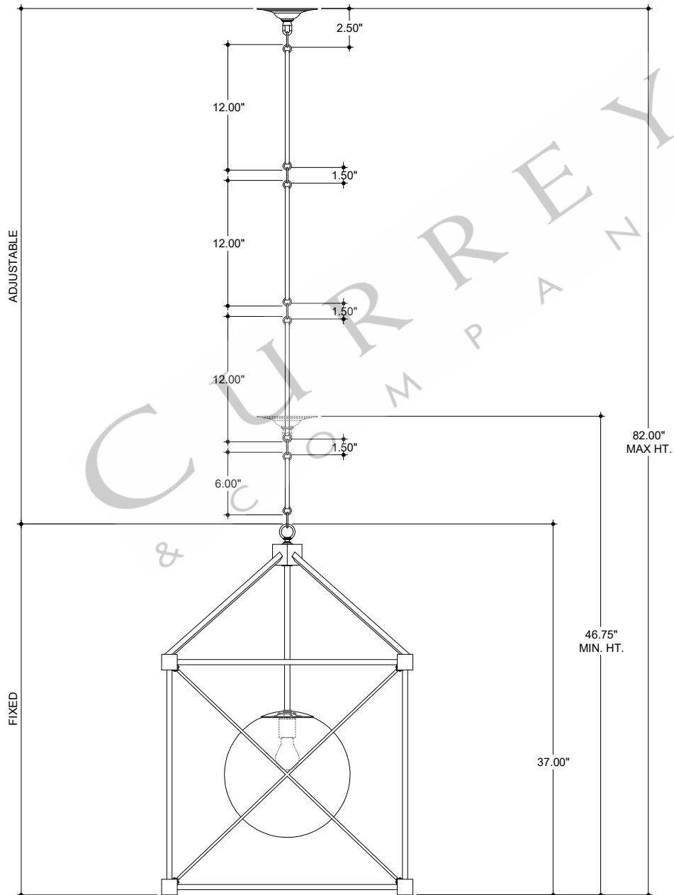
FRONT VIEW
