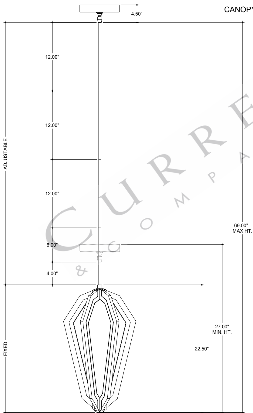
FRONT VIEW
