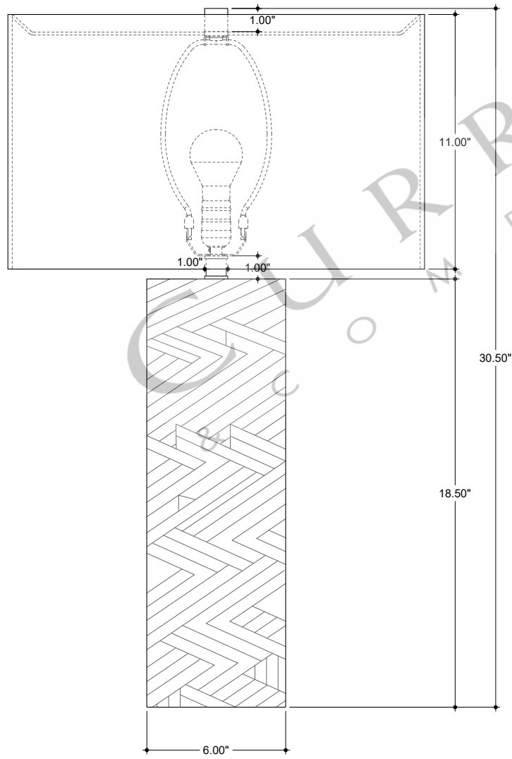
FRONT VIEW
