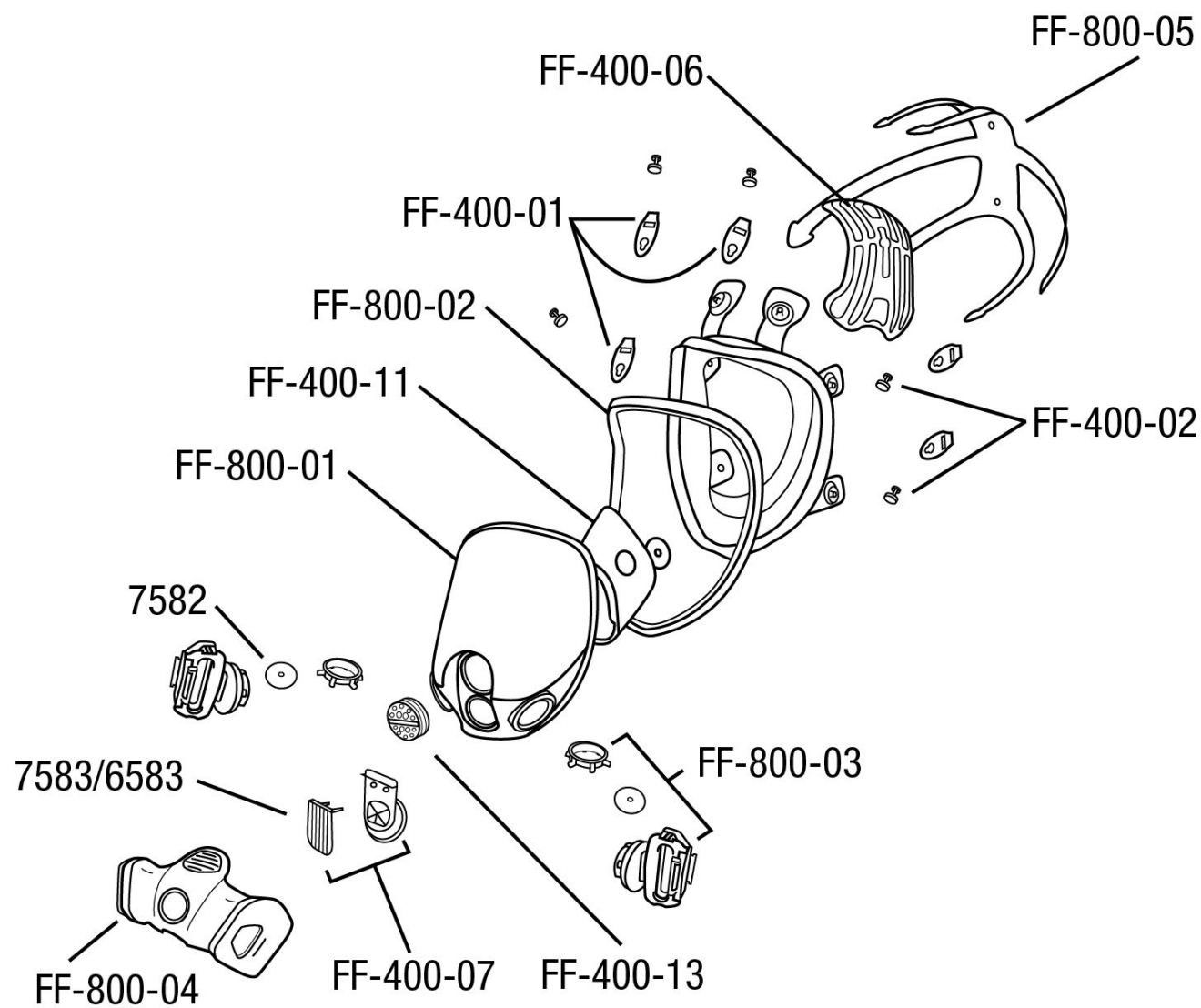
Figure 1: FF-800 Exploded View
