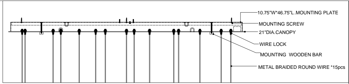
CANOPY DETAIL
