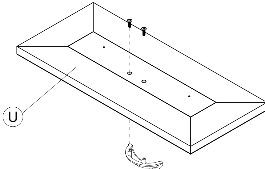
Handle
