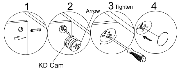
KD Cam
