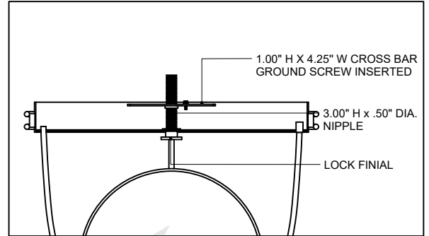
CANOPY DETAIL
