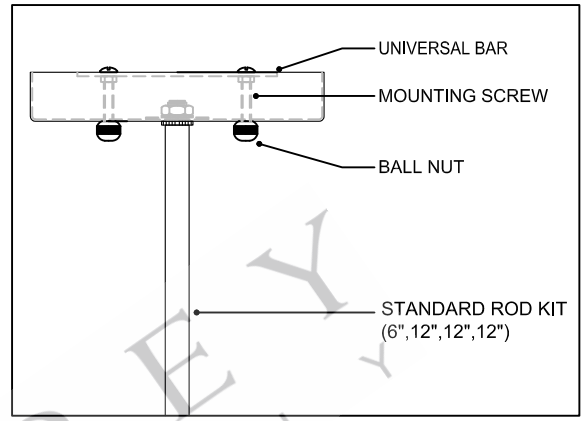
CANOPY DETAIL
