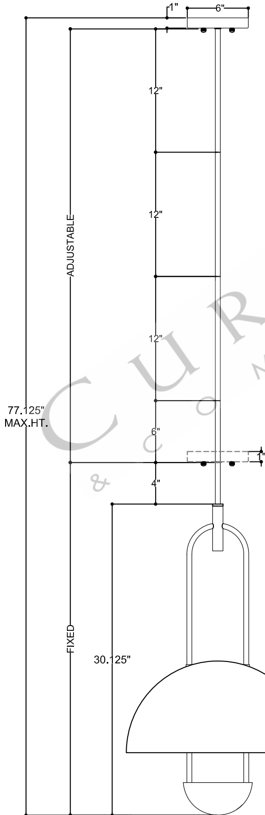
FRONT VIEW
