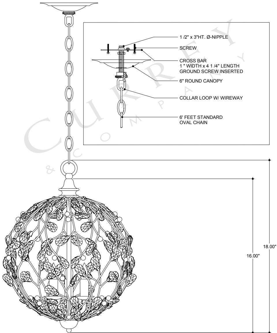
FRONT VIEW
