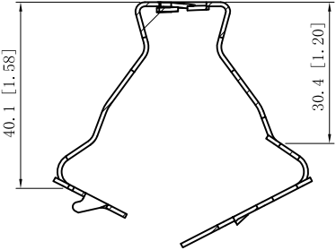
CUTAWAY VIEW C-C
