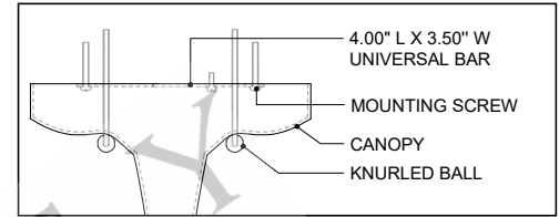
CANOPY DETAIL
