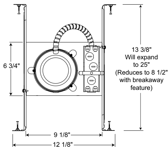
4 1/2" CEILING CUTOUT
