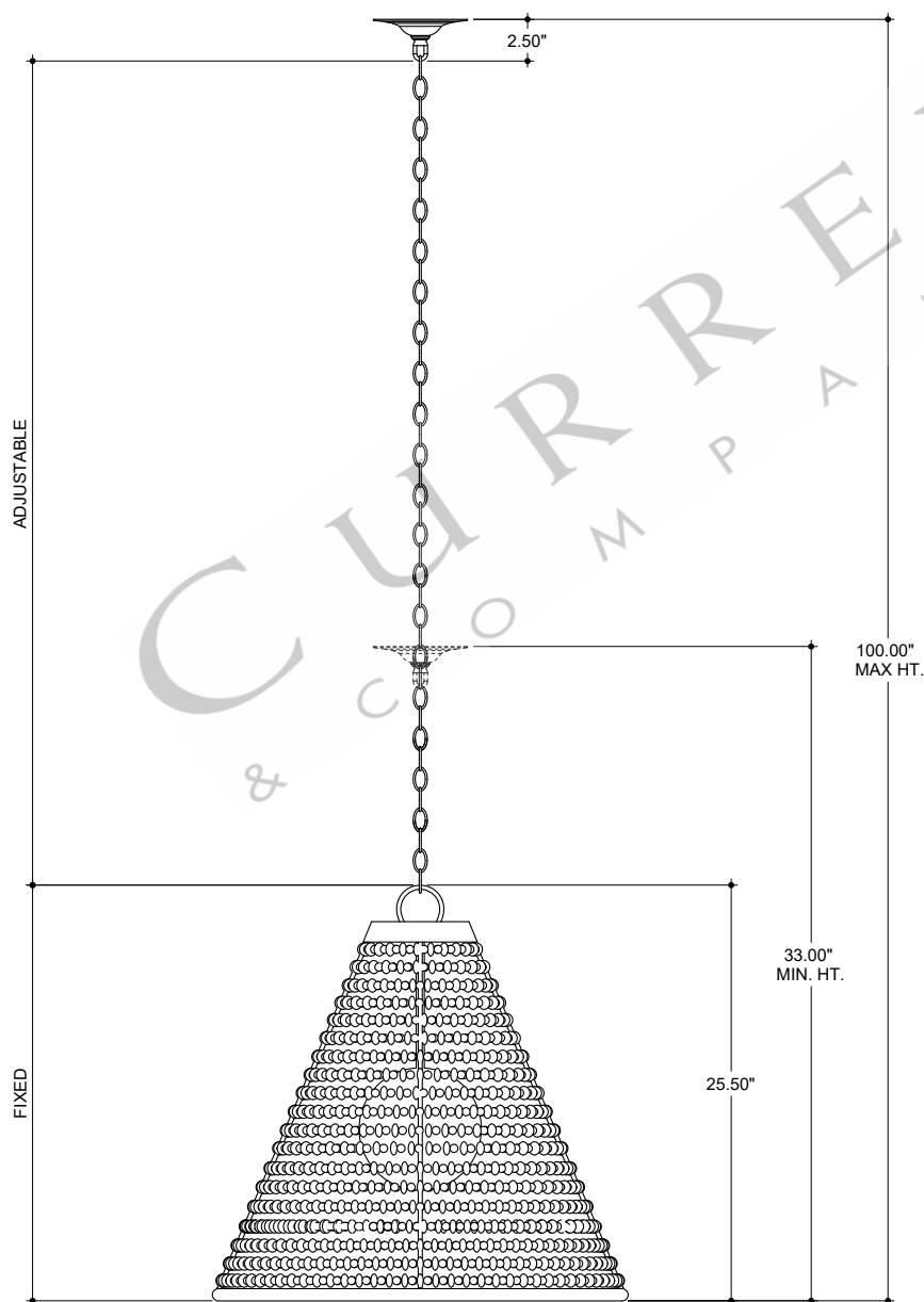
FRONT VIEW
