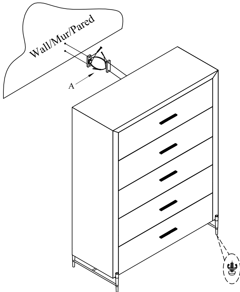
Adjustable leveler
