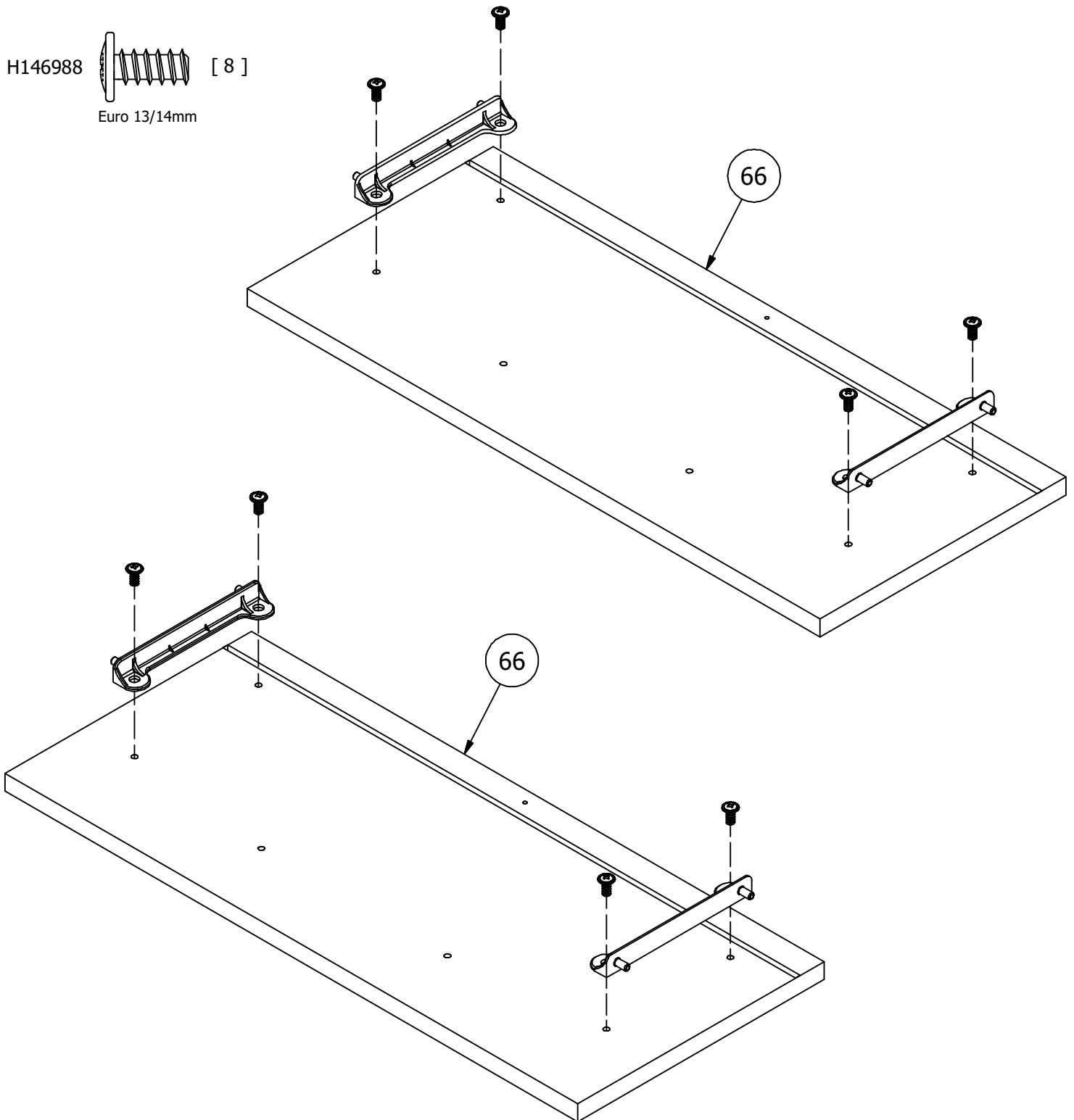
Drawer Bracket
