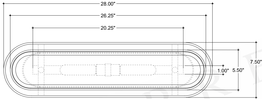
TOP VIEW
