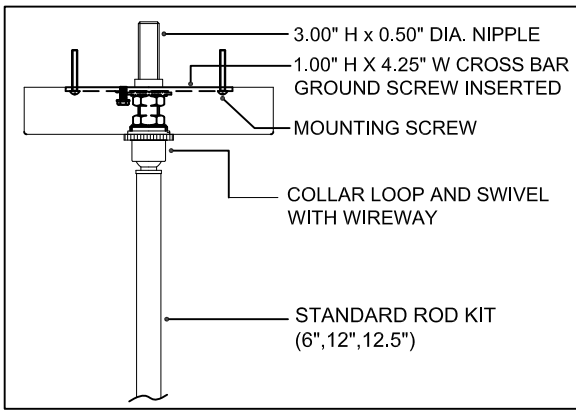
CANOPY DETAIL
