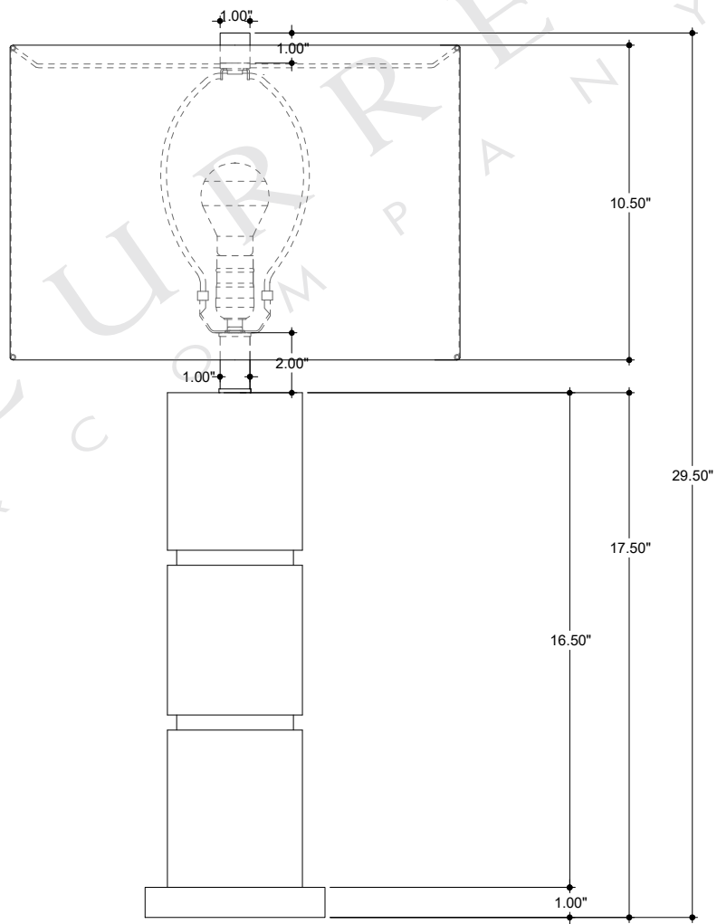
FRONT VIEW
