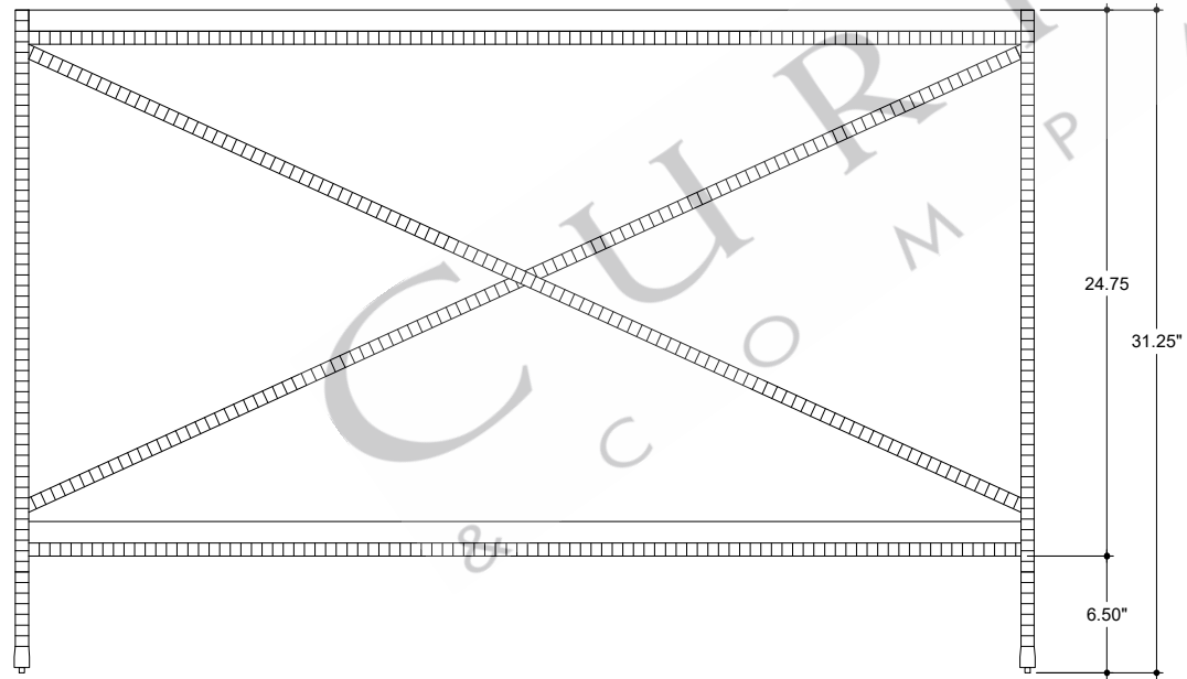
FRONT VIEW
