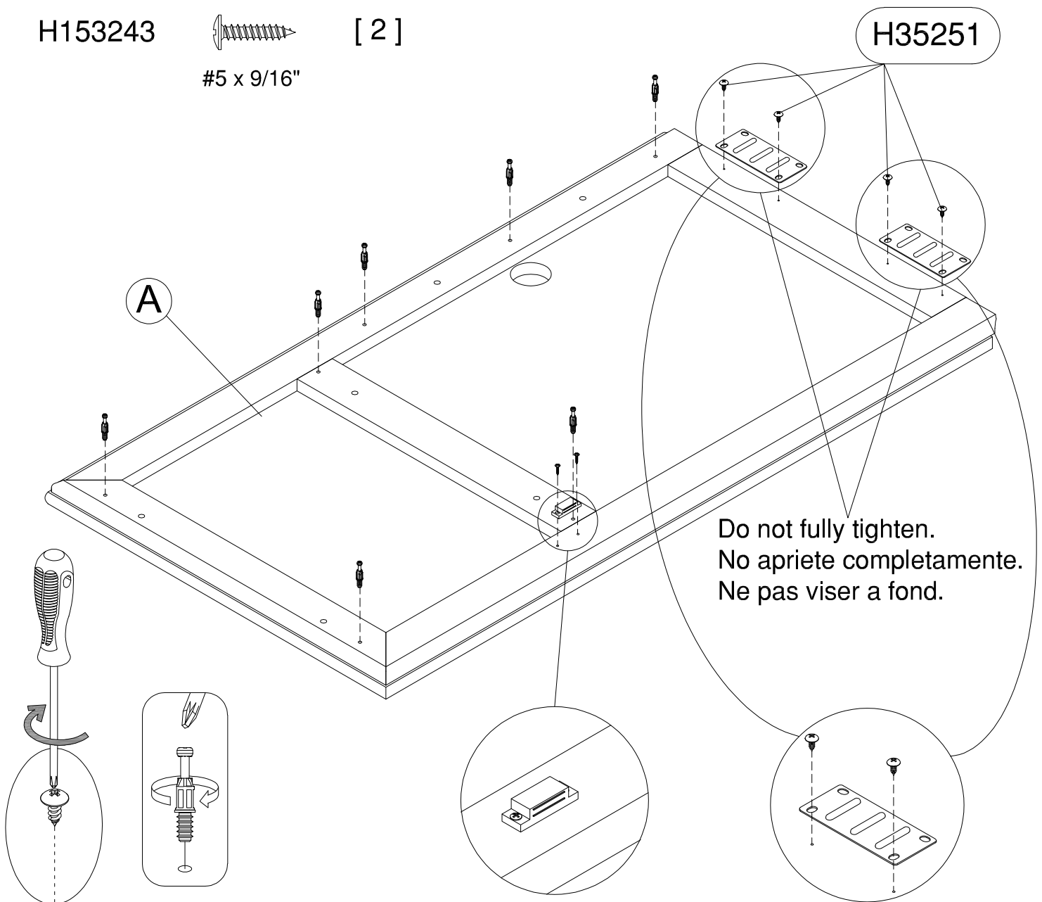
Magnetic Catch
