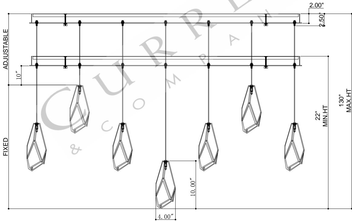
FRONT VIEW
