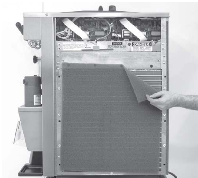
Figure 28. Condenser and Filter
