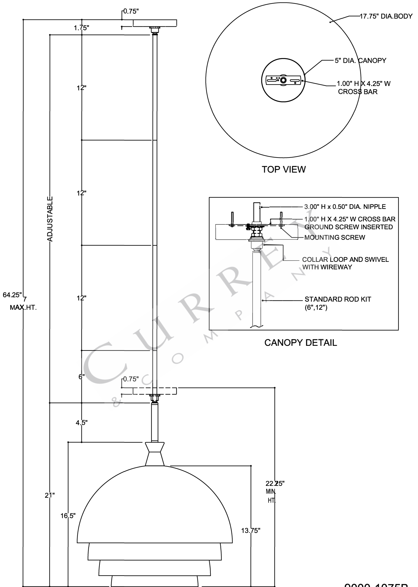
FRONT VIEW
