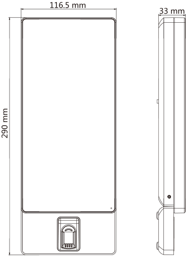
Figure E-1 Device with Fingerprint Module
