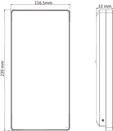
Figure E-2 Device without Fingerprint Module
