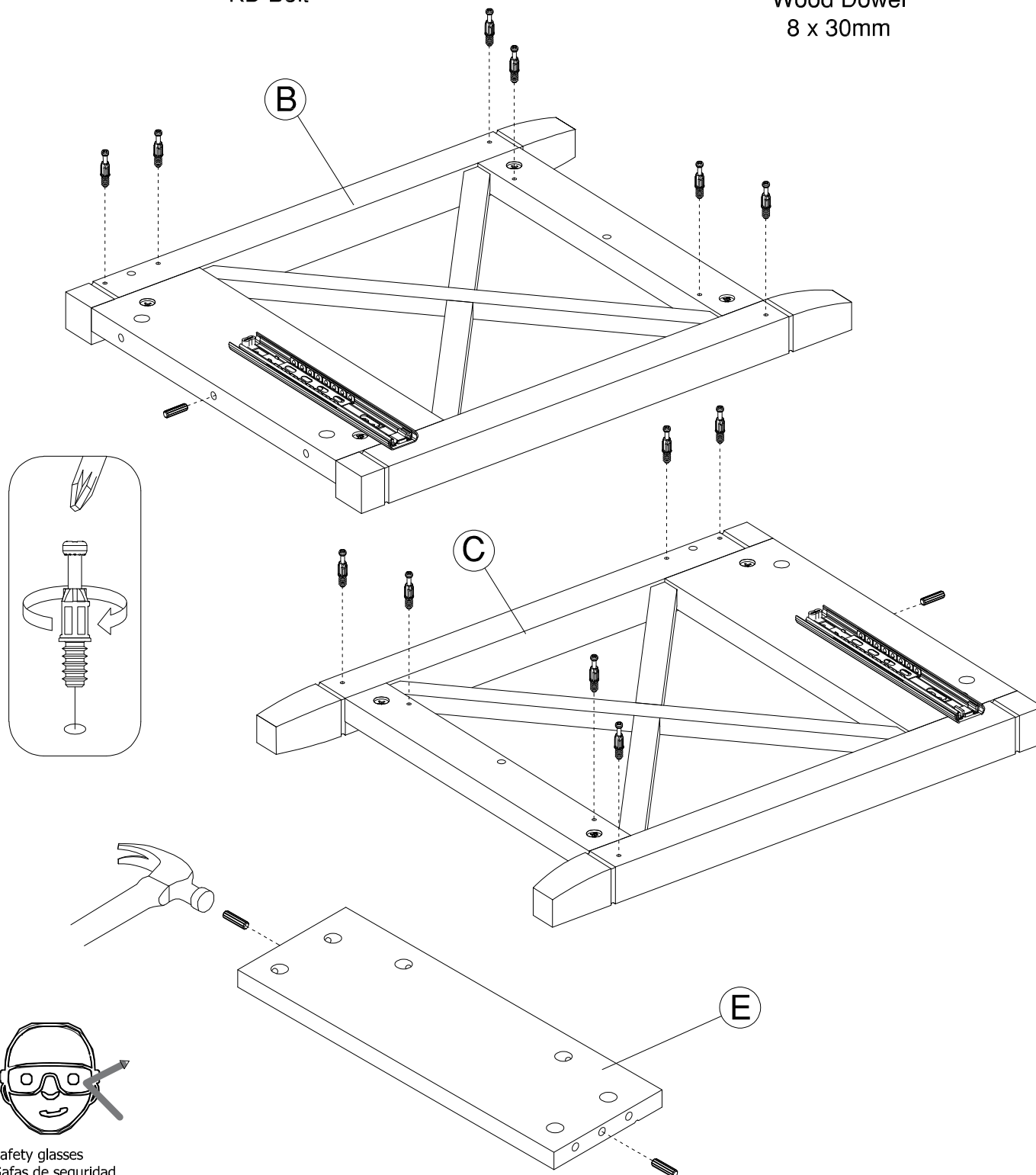
KD Bolt
