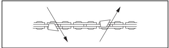
Figure 21 Filing Cutters
