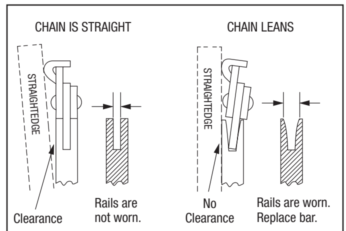
Figure 15 Checking Rails for Wear
