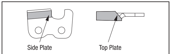
Figure 24 Filing Cutters
