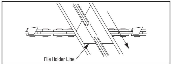
Figure 22 Filing Cutters
