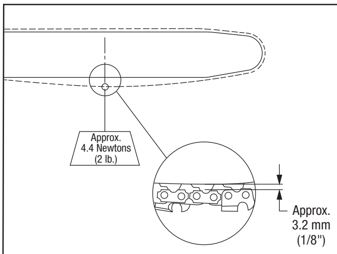
Figure 14 Proper Chain Tension
