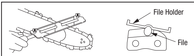
Figure 20 Filing Cutters
