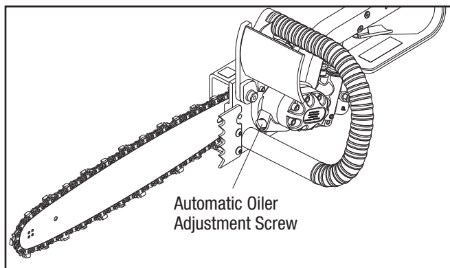
Figure 13 Automatic Oiler Adjustment Screw
