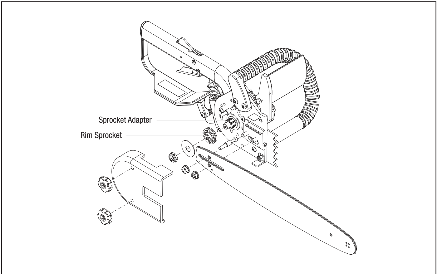
Figure 16 Rim Sprocket and Sprocket Adapter
