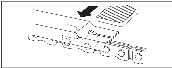
Figure 18 Lowering Depth Gauges
