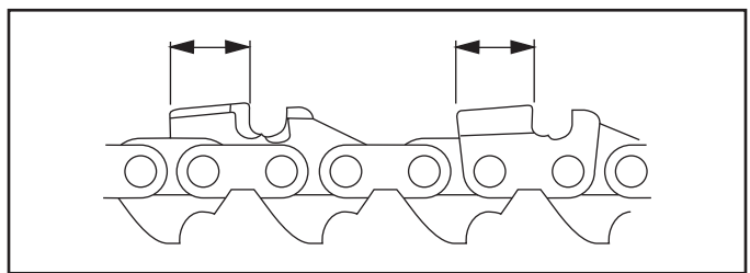
Figure 23 Filing Cutters
