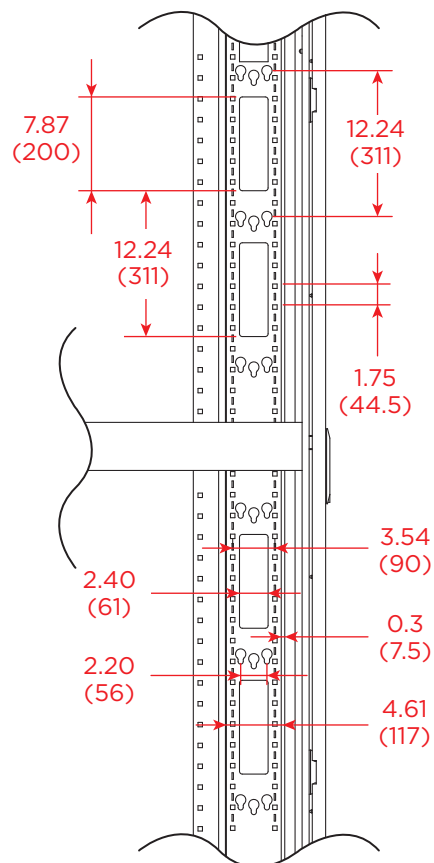
DETAIL-A
