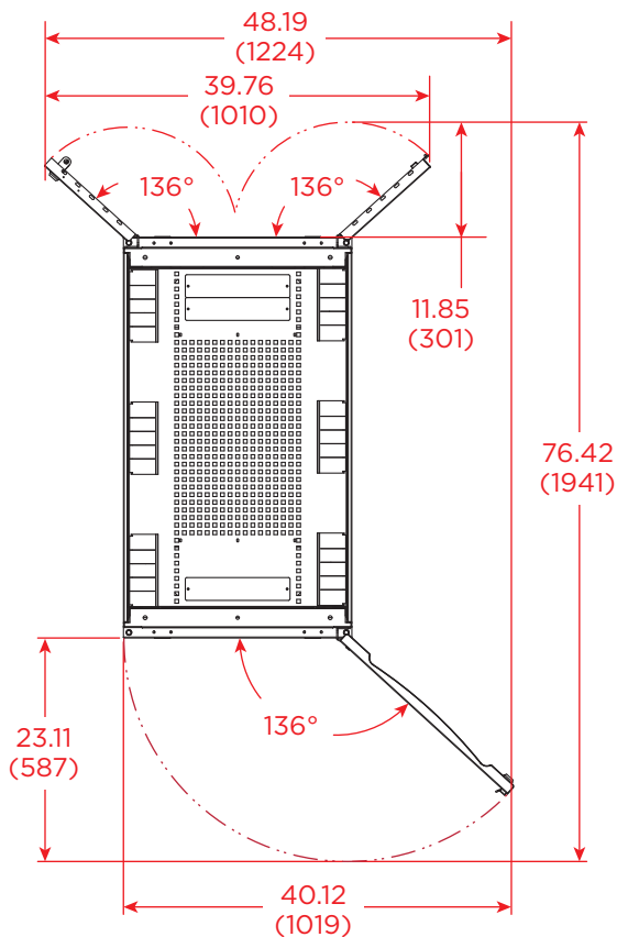
TOP VIEW (DOORS FULLY OPEN)
