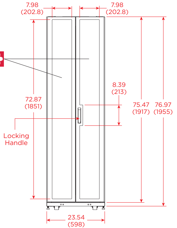
REAR VIEW
