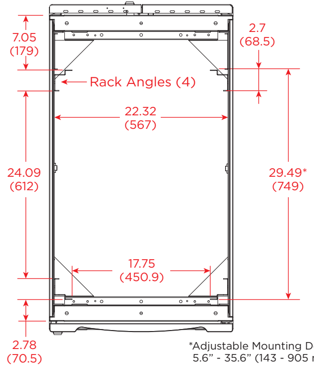
TOP VIEW W/O ROOF PANEL
