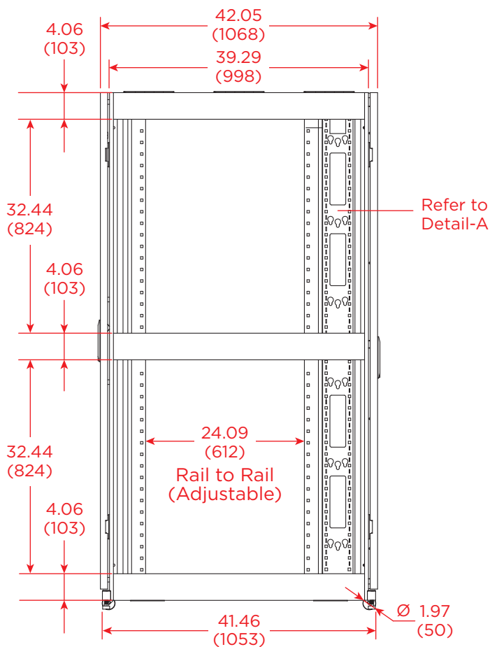
SIDE VIEW W/O SIDE PANELS
