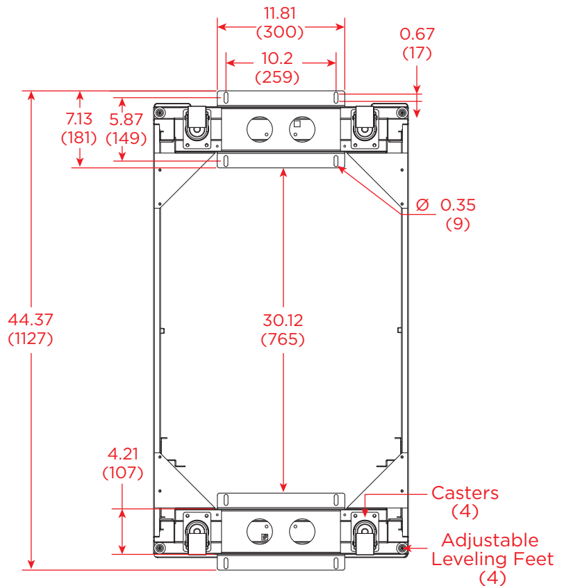
BOTTOM VIEW W/ SHIPPING BRACKETS
