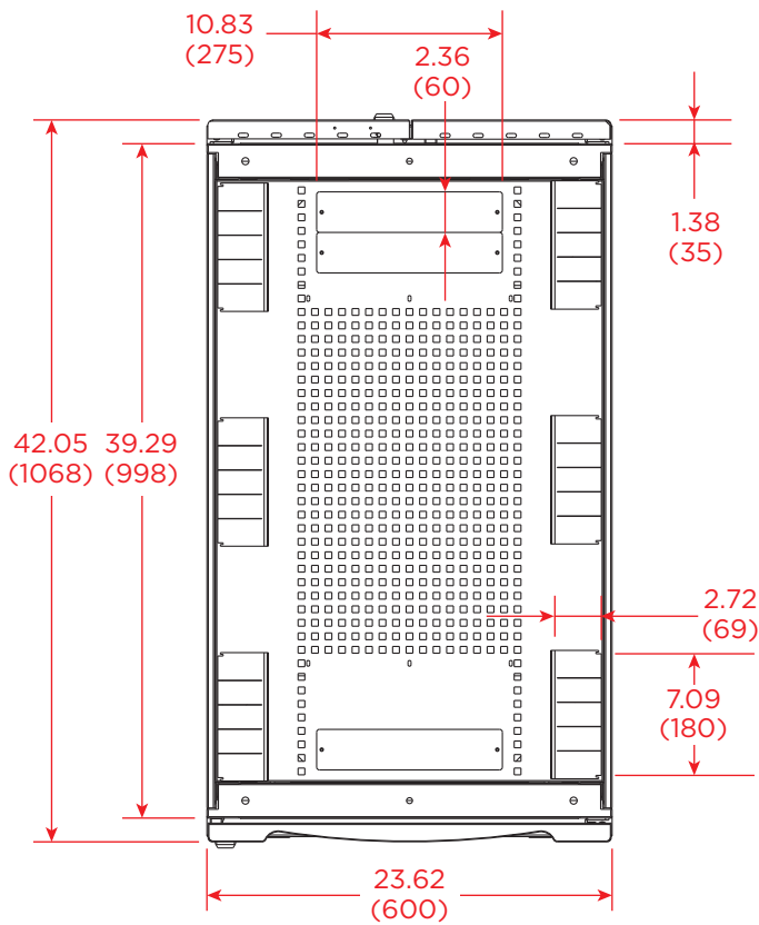
TOP VIEW
