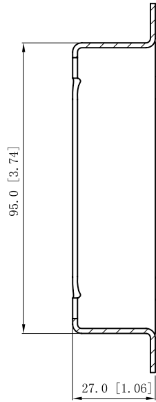
CUTAWAY VIEW B-B
