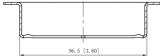
CUTAWAY VIEW A-A
