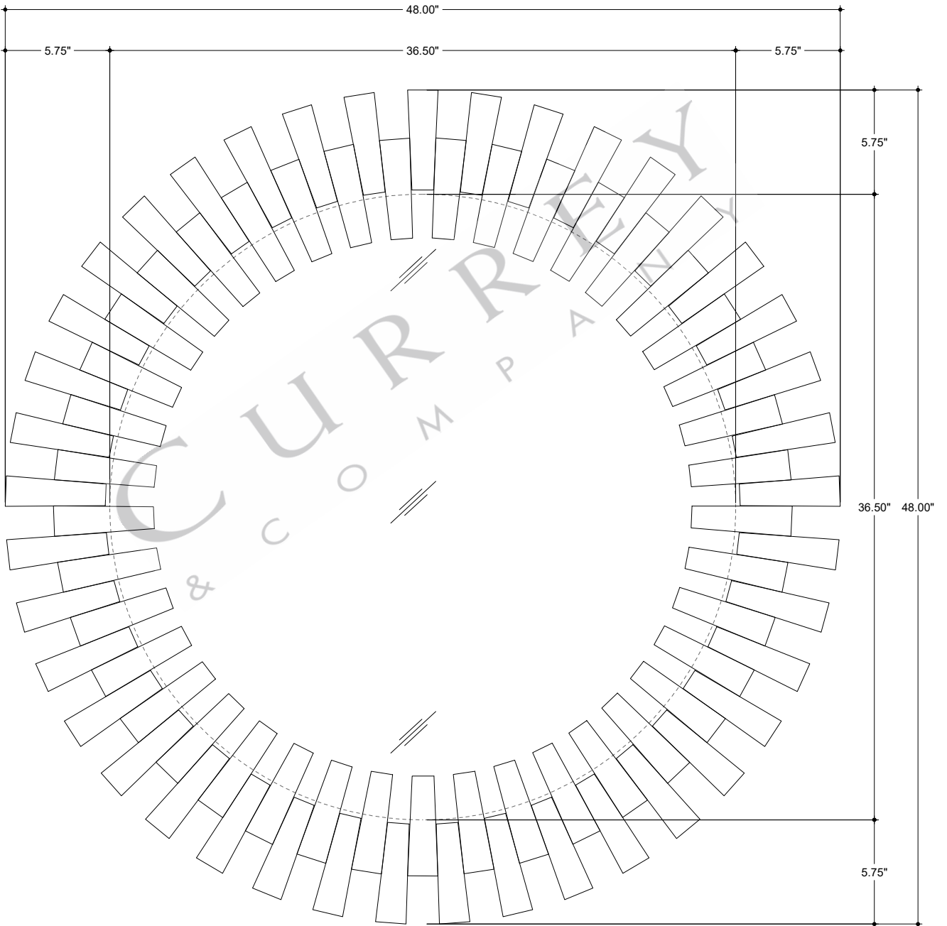
FRONT VIEW
