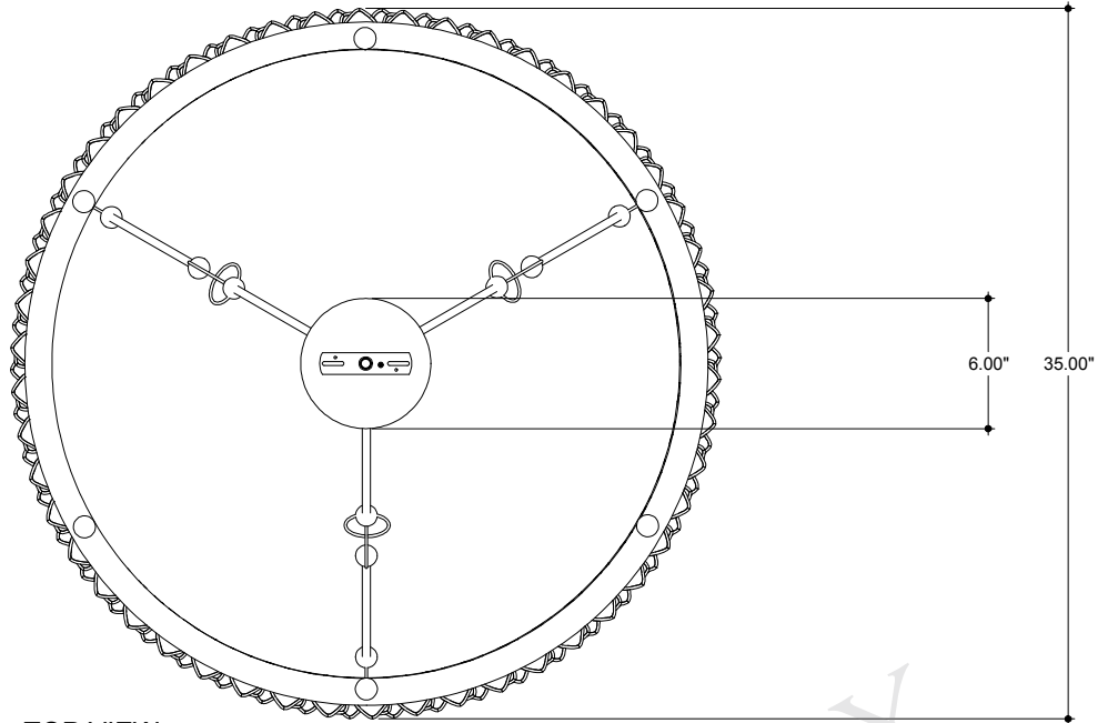
TOP VIEW
